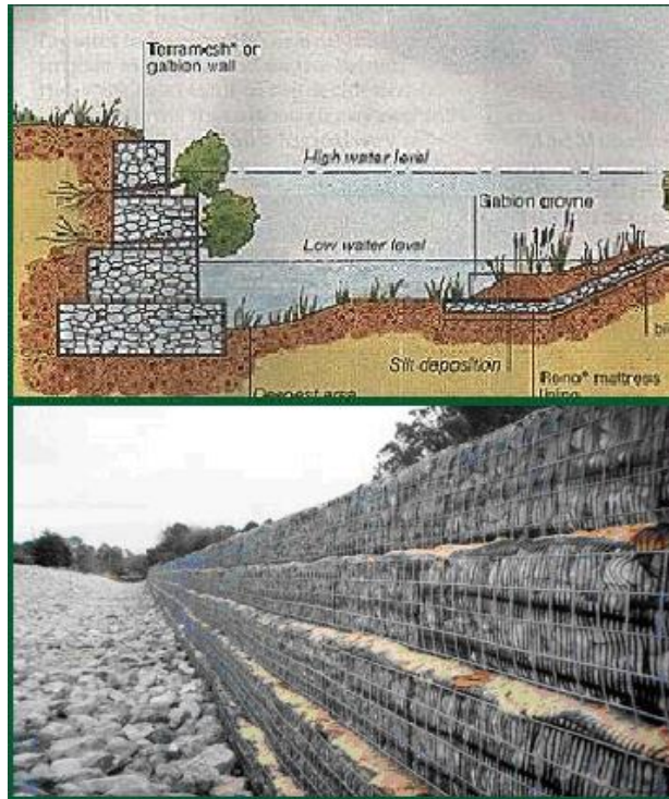
Gabion Wall
